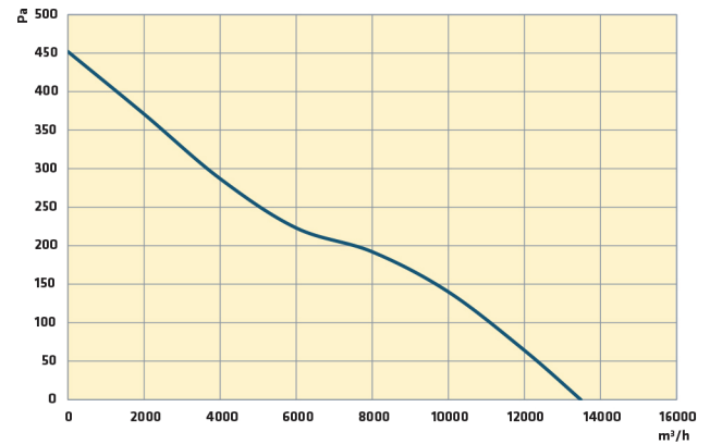
T/CC-ATX 630-5-30 T4 1,10 kW
