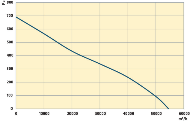
T/CC-ATX 1000-5-40 T4 7,50 kW
