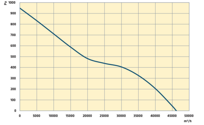
T/CC-ATX 900-8-40 T4 11,00 kW
