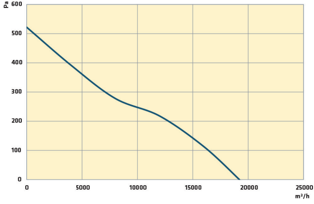
T/CC-ATX 710-5-30 T4 1,50 kW
