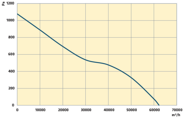
T/CC-ATX 1000-8-40 T4 15,00 kW
