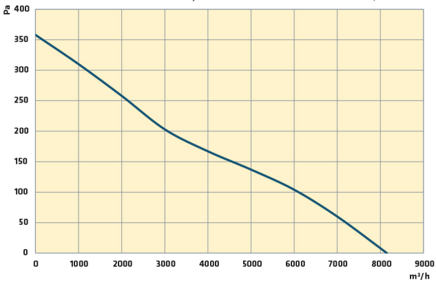
T/CC-ATX 560-5-25 T4 0,75 kW
