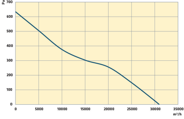
T/CC-ATX 800-5-35 T4 3,00 kW
